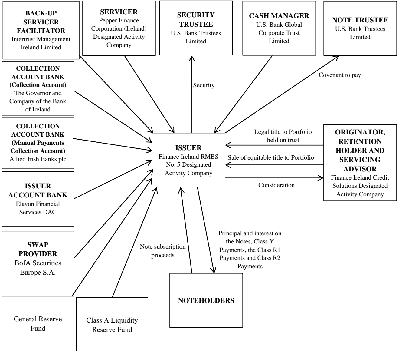
Figure 1 — Transaction Structure
